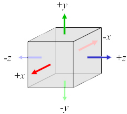
Figure 12: This figure shows, how an ambient cube looks like, schematically. A single color value for each face determines the lightflow along this direction through this volume in space. Image taken from [McT04]; see section 5.
