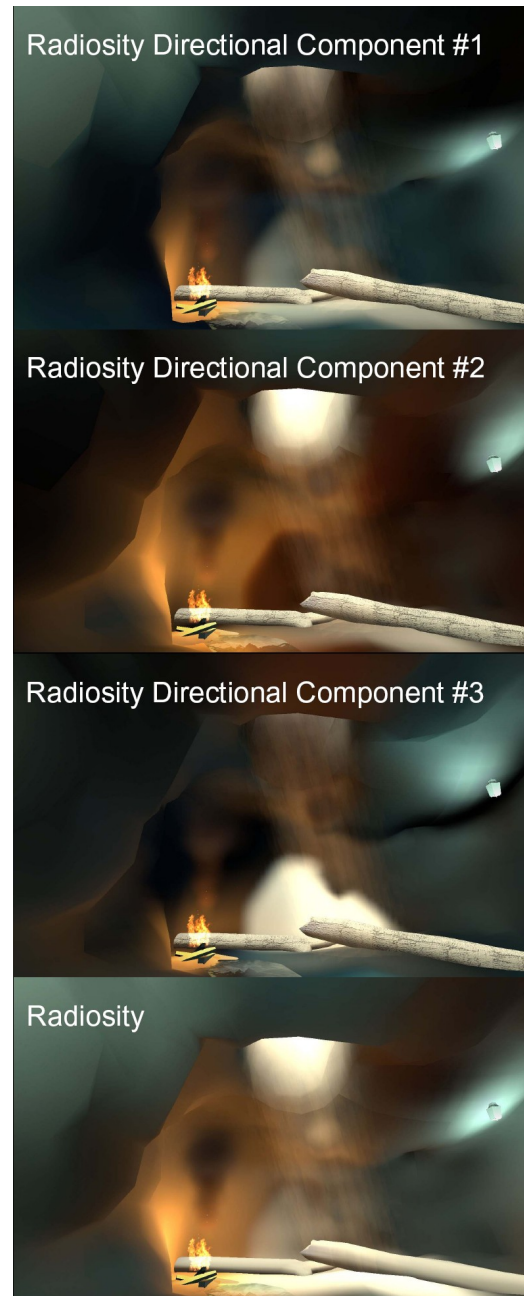
Figure 8: The three directional components in comparison to a traditional radiosity solution, which can be obtained by blending the three directional component-lightmaps. Each of the directional components is a radiosity solution with the hemicube placed on the same patch but each time facing along another basis vector. Through the three lightmaps directional dependencies are preserved and can therefore be used together with normal maps for elaborated shading effects on surfaces (see figure 9). Image(s) taken from [McT04]; see section 4.5.
