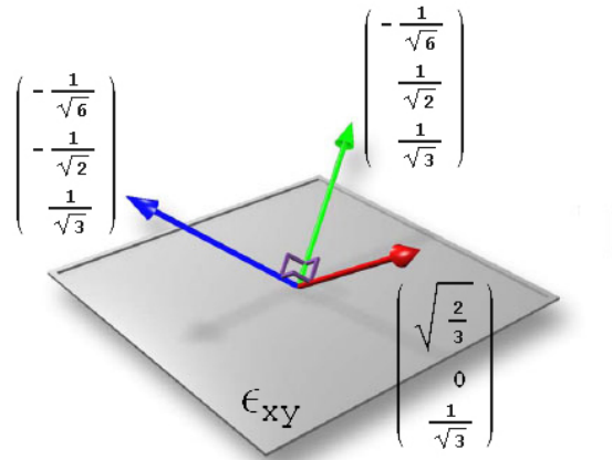
Figure 3: Basis for radiosity normal mapping. Note that the basis vectors form a cartesian coordinate system, where each two basis vectors are orthogonal to each other. Image taken from [McT04] (slightly modified); see section 4.1.
