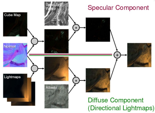
Figure 7: Schematic overview for how the individual parts from several stages in the pipeline are combined to form the desired result. The upper half shows the paths for the specular part, the lower half deals with the diffuse component - this is where directional lightmaps are used. Image composition is from left to right. Image taken from [McT04] (slightly modified); see section 4.5.
